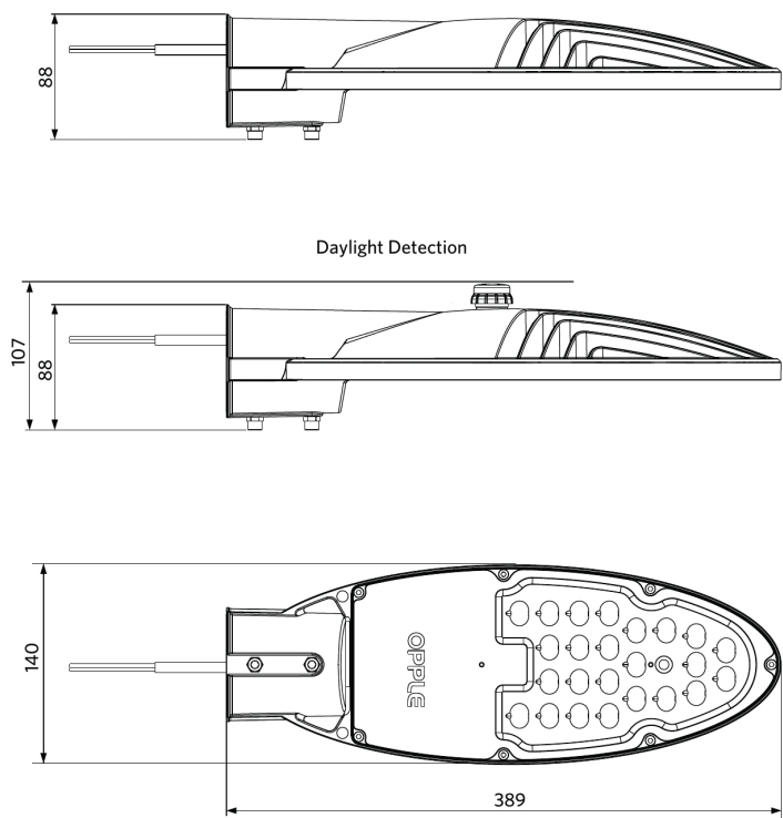
LEDStreet-SE-ExtensionCable
