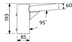
LEDStreetlight Pole-Top-76-Adapter-60
