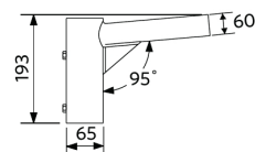
LEDStreetlight Pole-Top-60-Adapter-60
