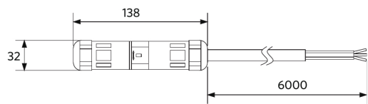
LEDStreet-SE-ExtensionCable
