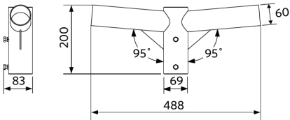
LEDStreetlight Pole-Top-60-Adapter-2x60
