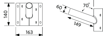
LEDStreetlight Wall-Bracket-60
