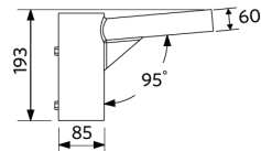
LEDStreetlight Pole-Top-76-Adapter-60
