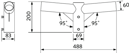
LEDStreetlight Pole-Top-60-Adapter-2x60
