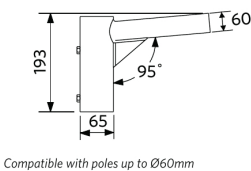
LEDStreetlight Pole-Top-76-Adapter-60
