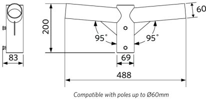
LEDStreetlight Wall-Bracket-60
