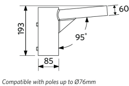
LEDStreetlight Pole-Top-60-Adapter-2x60
