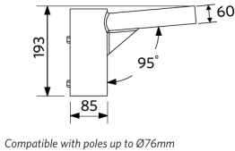
LEDStreetlight Pole-Top-60-Adapter-2x60
