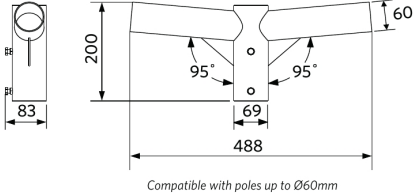
LEDStreetlight Wall-Bracket-60
