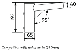
LEDStreetlight Pole-Top-76-Adapter-60
