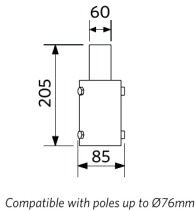
LEDStreetlight Pole-Top-60-Adapter-60
