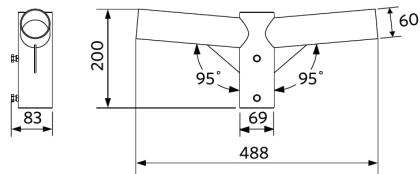
LEDStreetlight Pole-Top-60-Adapter-2x60
