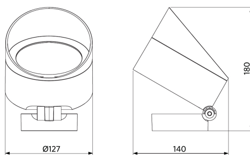
LEDSpotProjector-E Rd127
