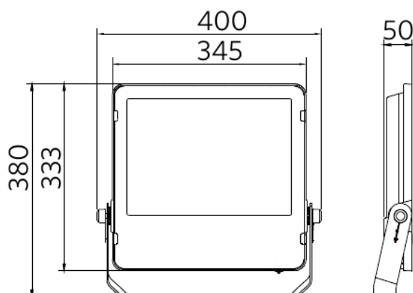
LEDflood-E3 Re345 200W
