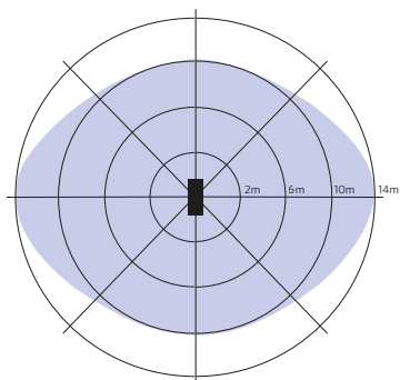
Asymmetric (ASY) Installation - Low Ceiling Suggested installation height 3m
