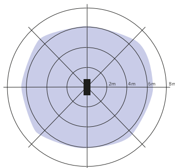
Round (RND) Installation - Low Ceiling Suggested installation height 3m
