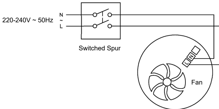
Fig.1 Continuous trickle (no manual boost). (The fan is internally fused)
