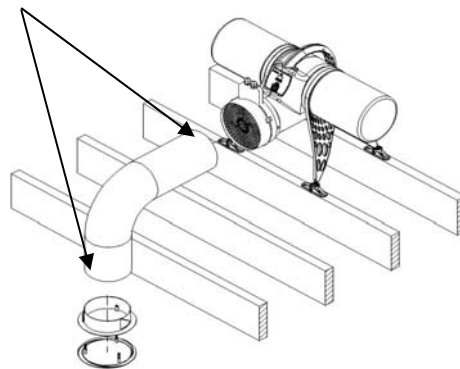
Fig. 8: Apply worm drive clips provided in positions shown
