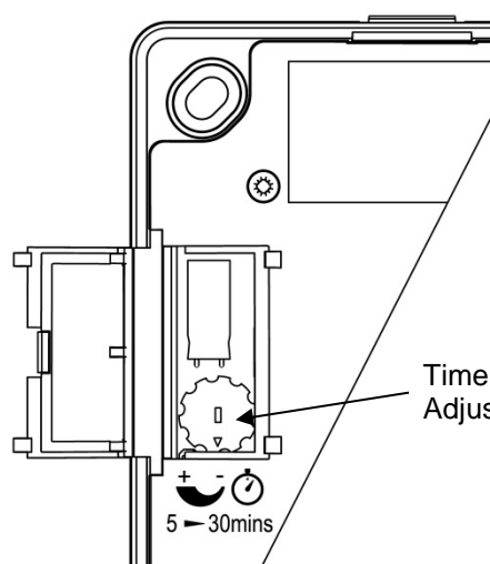
FIG. 5: PIR TIMER
