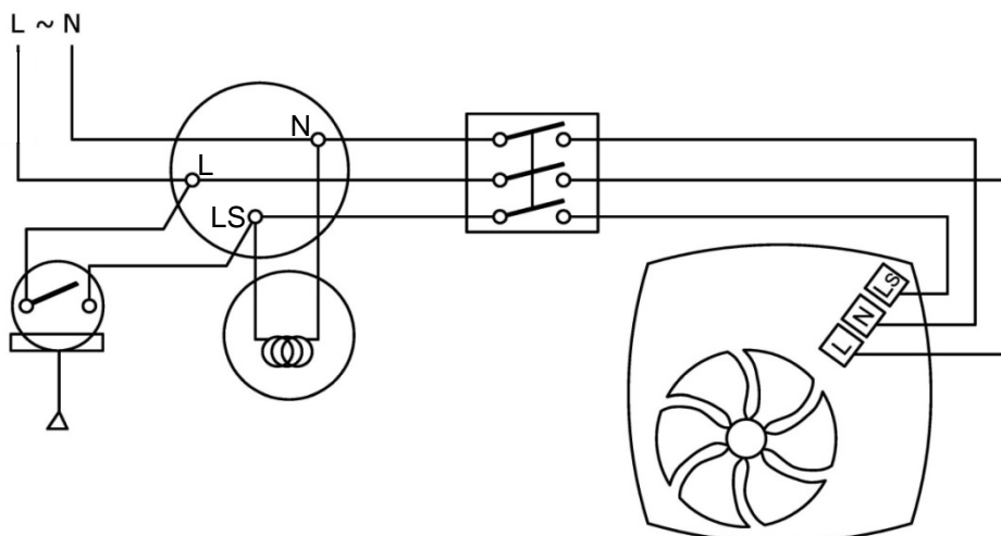
FIG. 5: PIR TIMER
